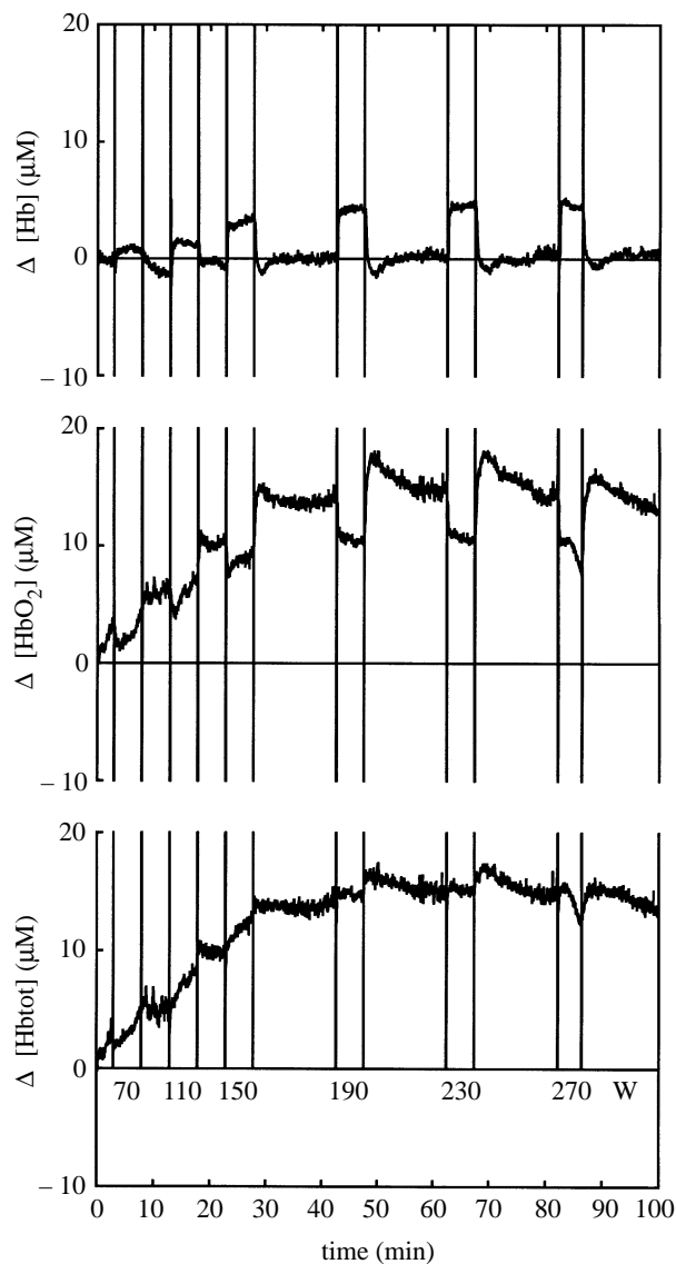
Figure 4. Effects of a series of square wave exercises on the quadriceps of an untrained cycling subject. Measurements performed with a NIR CWS (NIRO500). Sampling time: 2 s.
